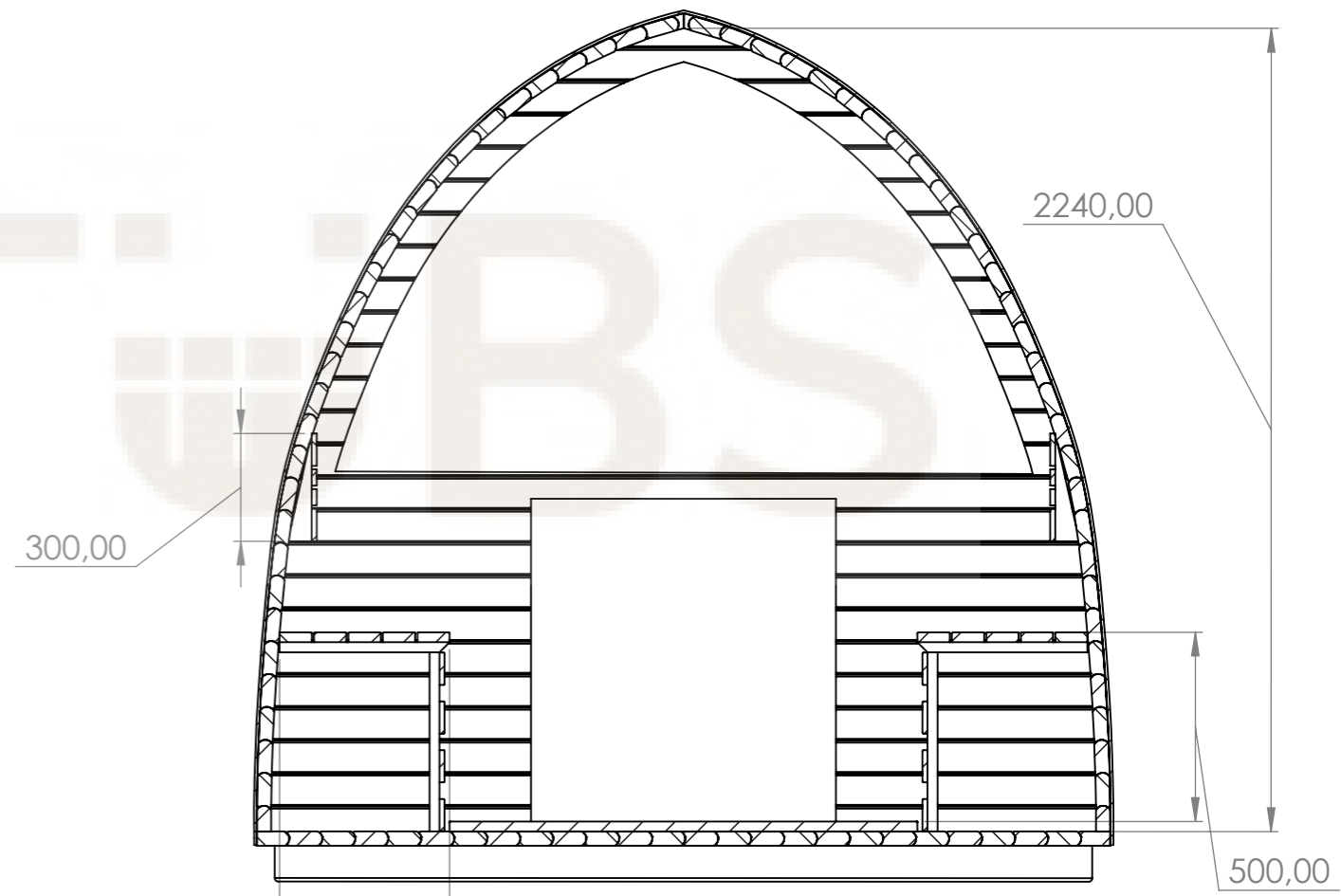
SECTION B-B
